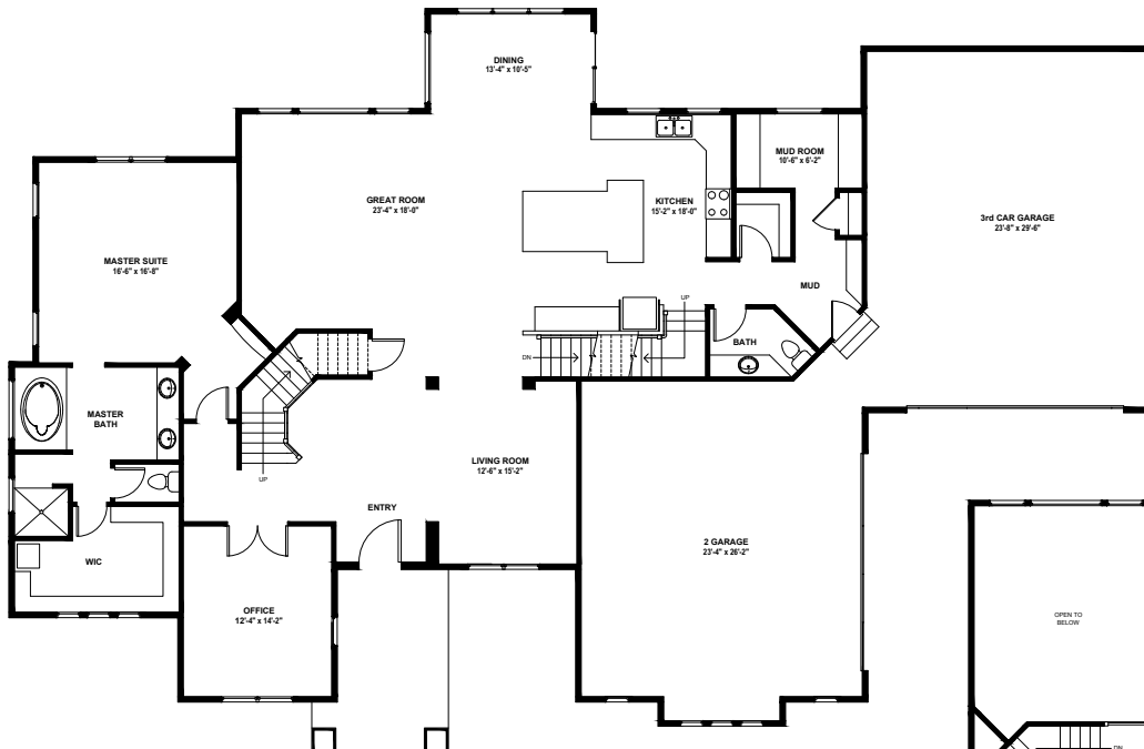
Main Level
